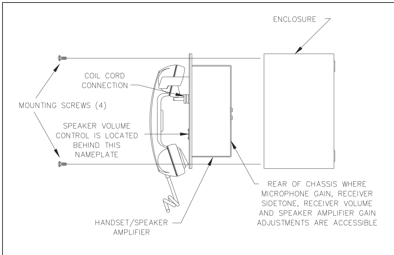
Figure 1. Installation and Adjustment Details
